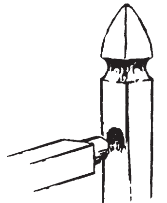
DOWELED END CONSTRUCTION
